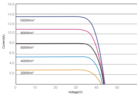
昊宇光伏I-V曲线图(590W)
